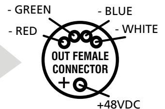
output connector rear side welding view
