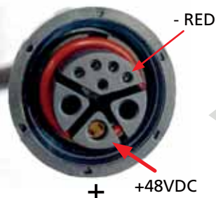
output connector front view
