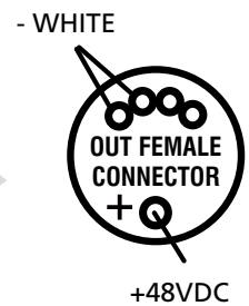
output connector rear side welding view
