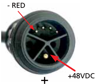
input connector front view
