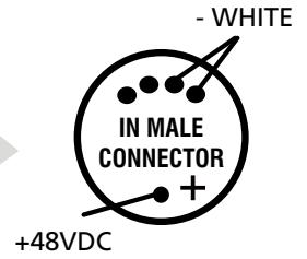
input connector rear side welding view
